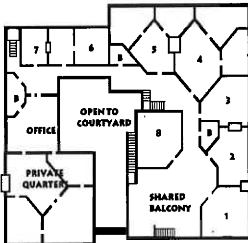
SECOND LEVEL
